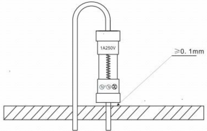
B、立式安装 Vertical installation
